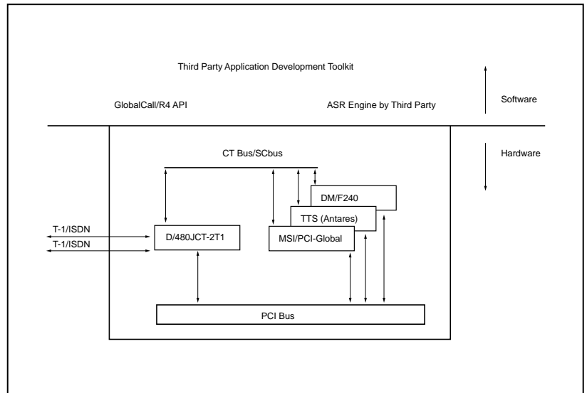
Terminate Configuration
