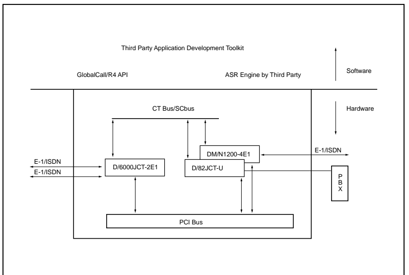
Drop-and-Insert Configuration
